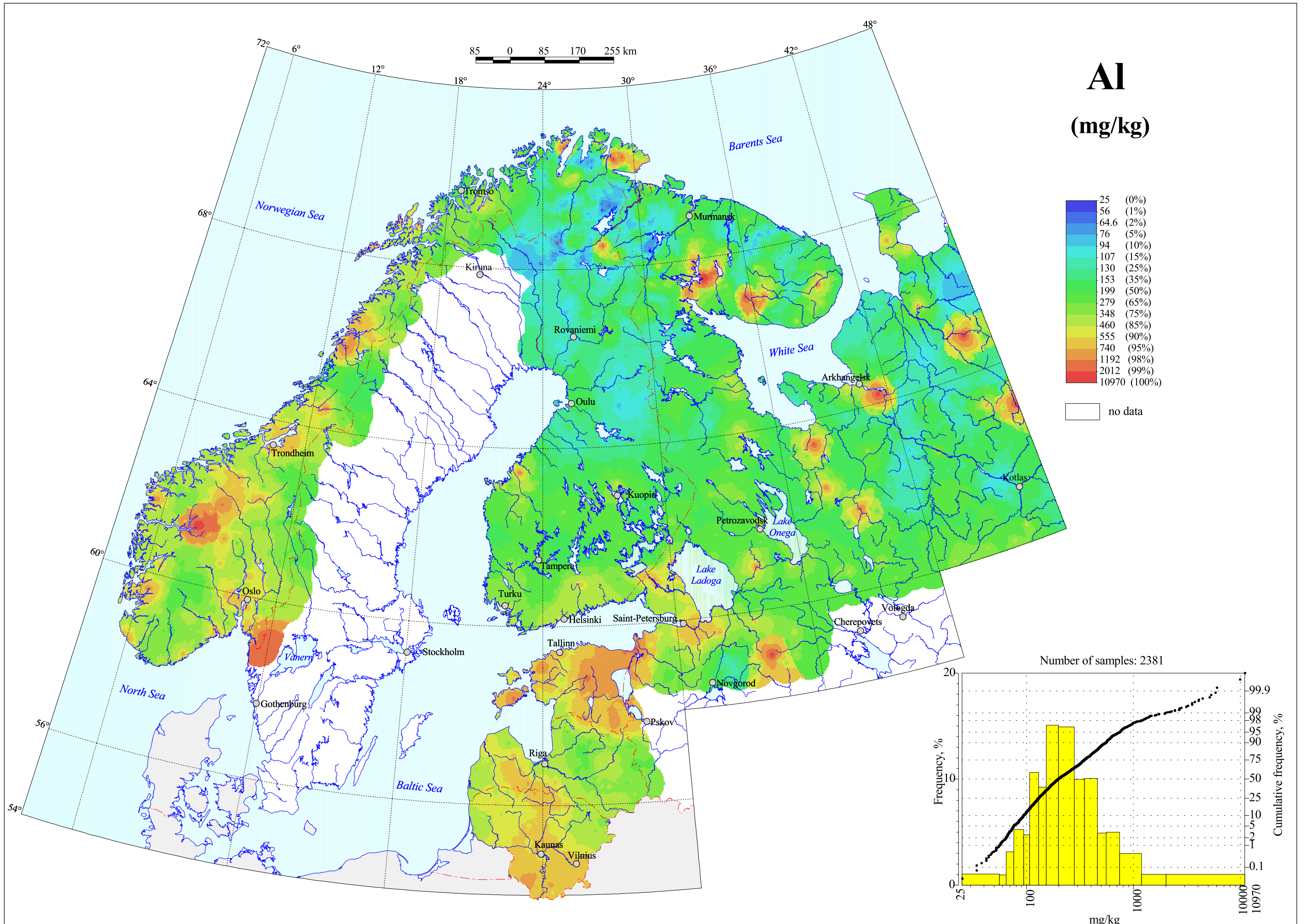
Aluminium in Terrestrial Moss, Total Content
